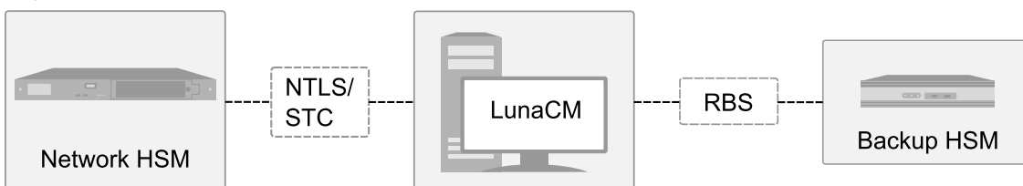
Figure 9: Remote Backup
