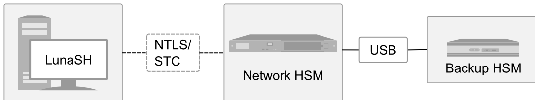
Figure 7: Centralized Local Backup
